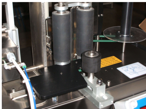
Rollers for 17mm bottles
